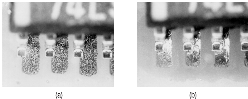
Figure 16: Optical photographs showing component alignments (a) before reflow and (b) after reflow in air for WS solder paste.
