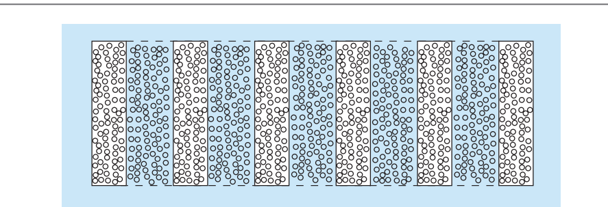
Figure 2: Schematic drawings showing “cross printing” of solder paste on trace area of a circuit board.
